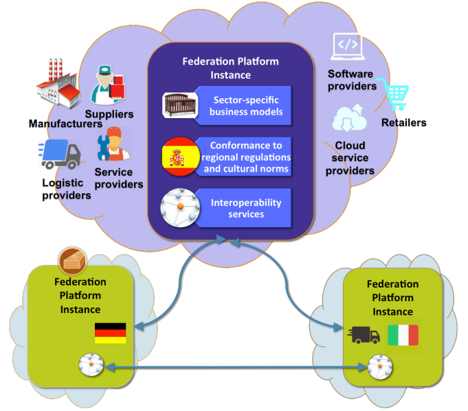
Fig. 1 NIMBLE federated collaboration network with sector-centric platform instances
